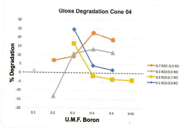
Figure 2. Documenting the washed degradation of several glazes based on boron and flux variation.
