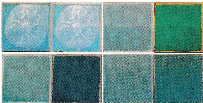
Figure 1. Above is an image of various non-durable cone 04 glazes exposed to the lemon test. On the left of each pair are the original samples, post-test. On the right are the same samples, with the color and saturation adjusted to make the acid etching more visible.
